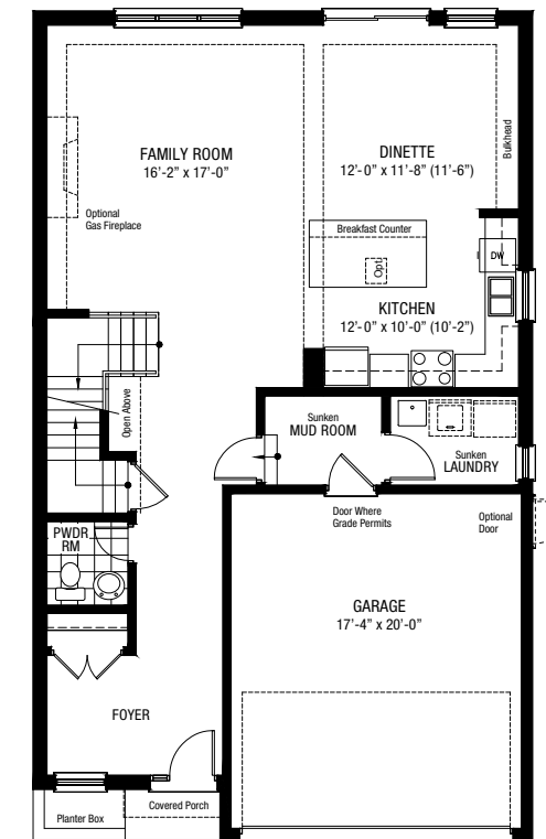
OPT. MAIN FLOOR WITH MUD ROOM
